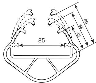
RackGuard (S) SLR, MLR, LLR
